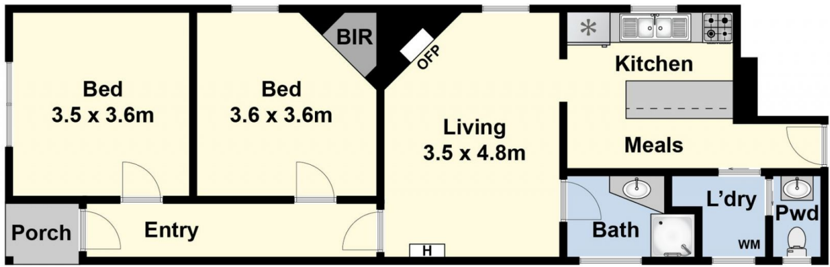
Ground Floor
