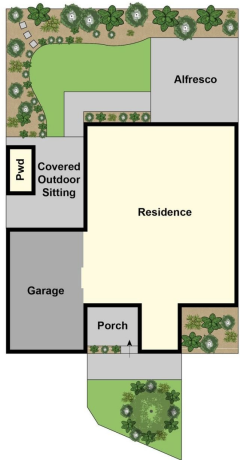
Site Plan
