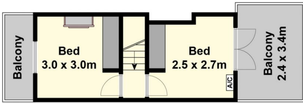
First Floor
