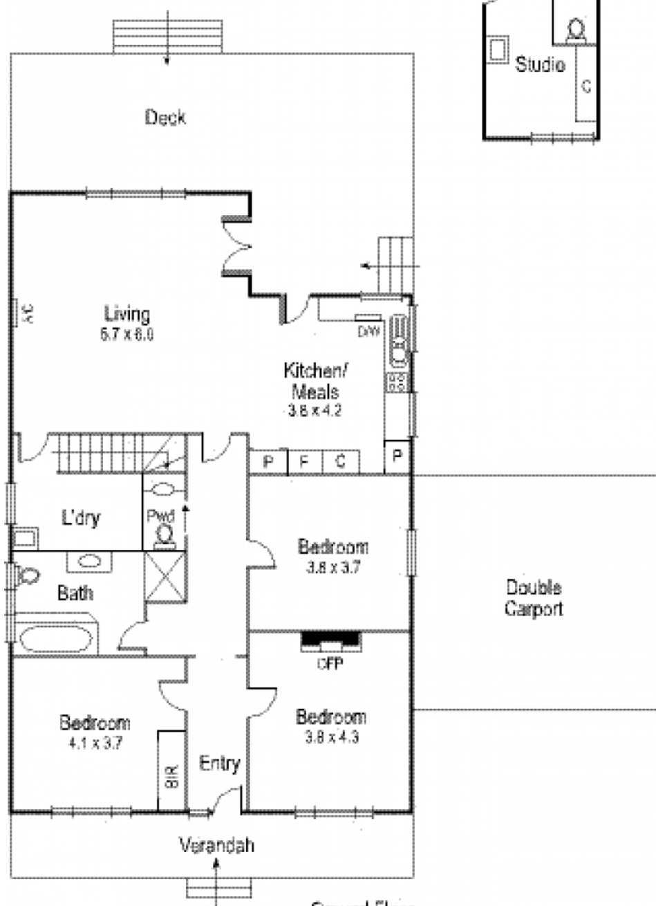
Ground Floor
